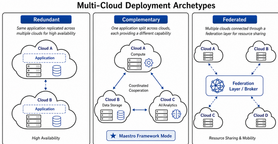
Figure 2.7: Multi-cloud deployment archetypes - redundant, complementary, and federated strategies - as classified by Petcu [37]. The Maestro framework operates in complementary mode.
