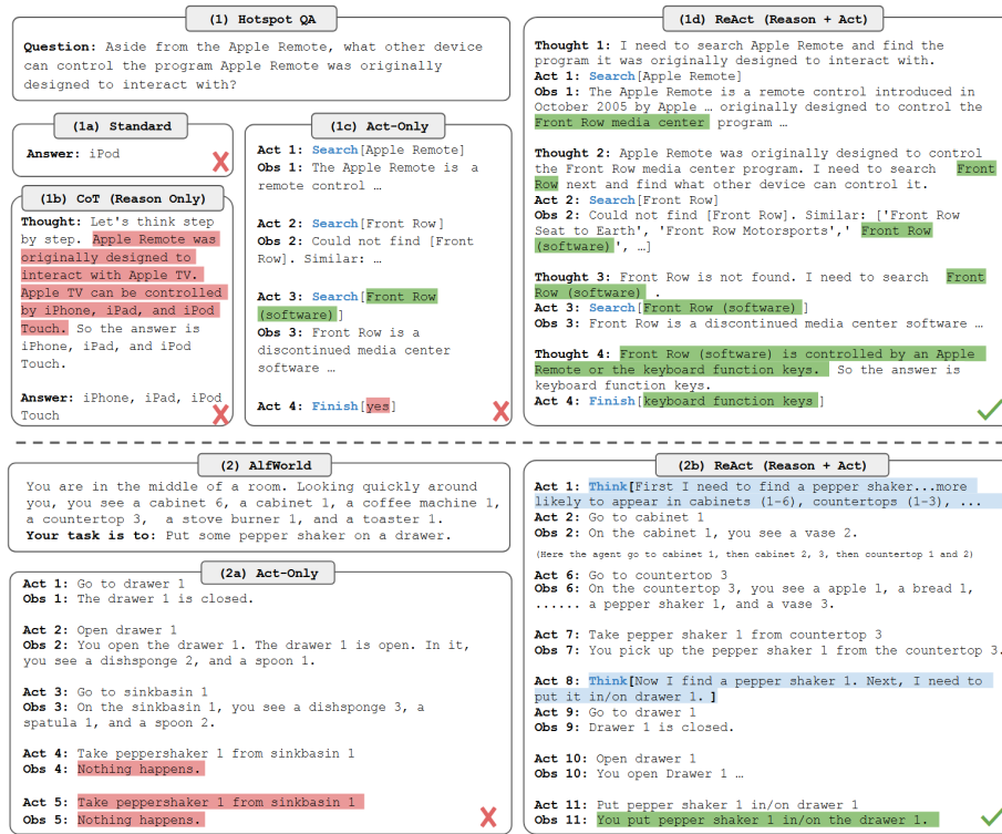
Figure 2.4: The ReAct reasoning loop interleaving Thought , Action , and Observation steps. Borrowed from [51].
