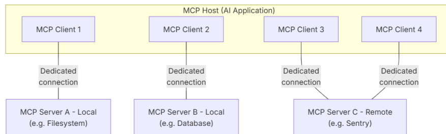
Figure 2.5: MCP architecture showing the Host, Client, and Server roles connected via JSON-RPC 2.0. Borrowed from [34].
