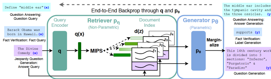
Figure 2.2: End-to-end RAG architecture combining a DPR retriever with a BART-large generator. Borrowed from [28].
